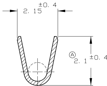
SECT. B-B
